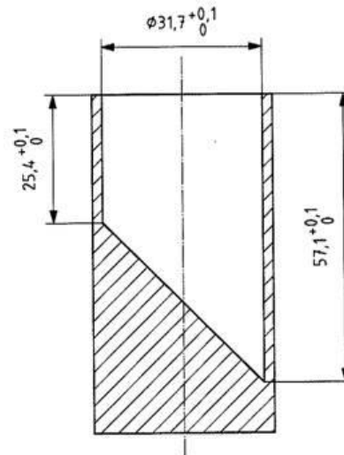
Small parts cylinder (dimensions in millimetres)
